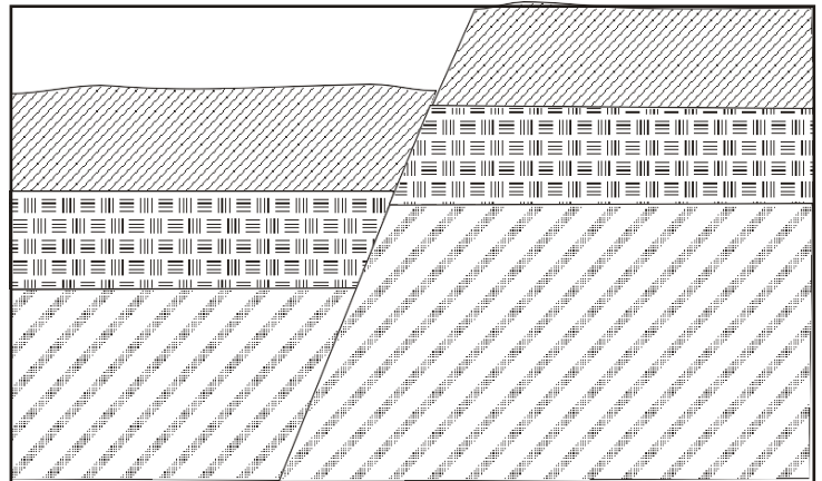
Diagram showing how the uplift thrust the western block upwards. The resulting dam held back the Murray and Goulburn, forming two lakes.
