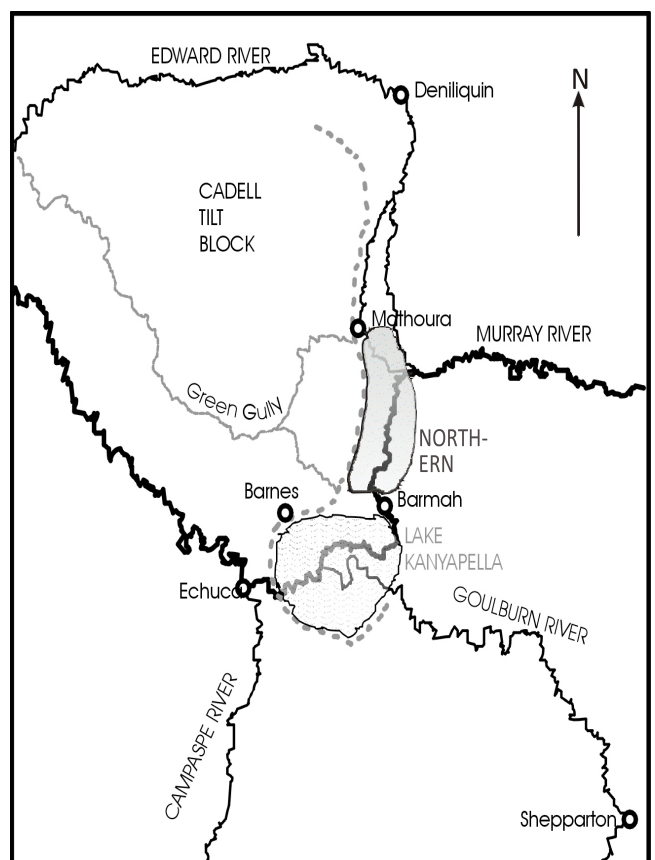
Map showing position of Cadell Fault (broken grey line) and ancient stream beds together with Lake Kanyapella and the northern lake. (After Bowler and Harford, 1966 and Stone T. 2007)
